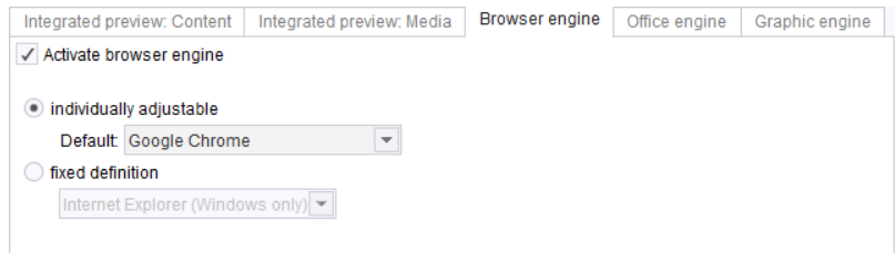
FirstSpirit ServerManager
