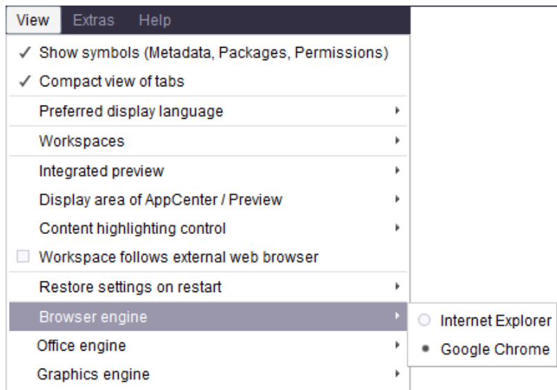
FirstSpirit SiteArchitect
