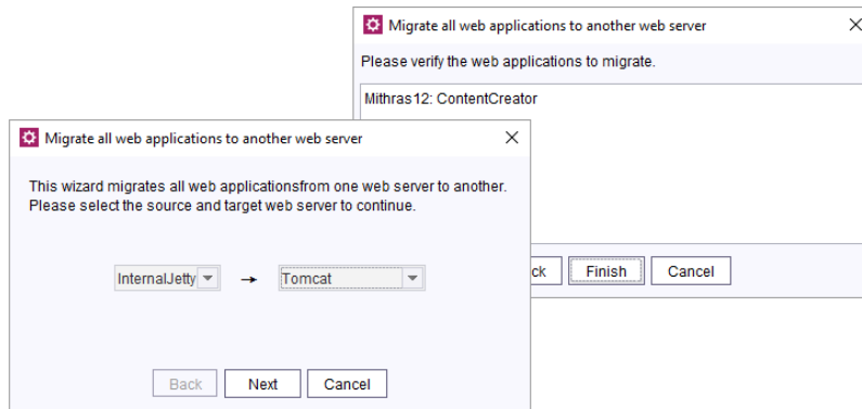
Migration wizard
