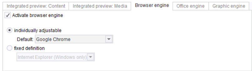
FirstSpirit ServerManager
