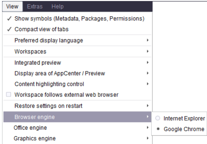
FirstSpirit SiteArchitect
